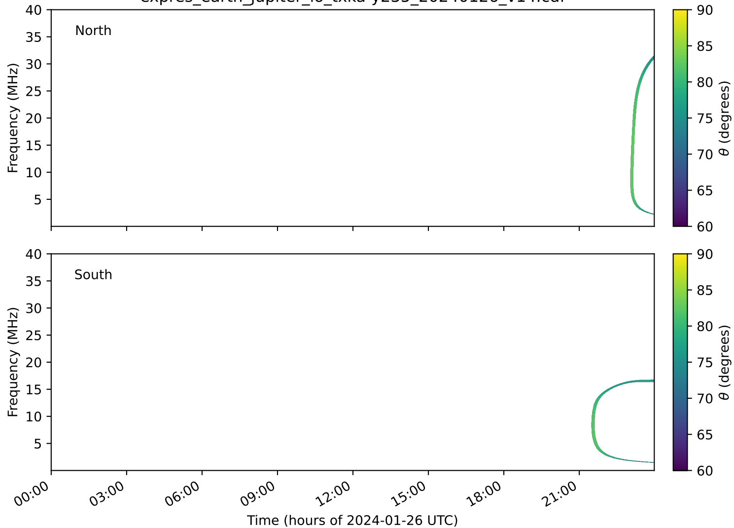
expres_earth_jupiter_io_txka-y235_20240126_v14.cdf
