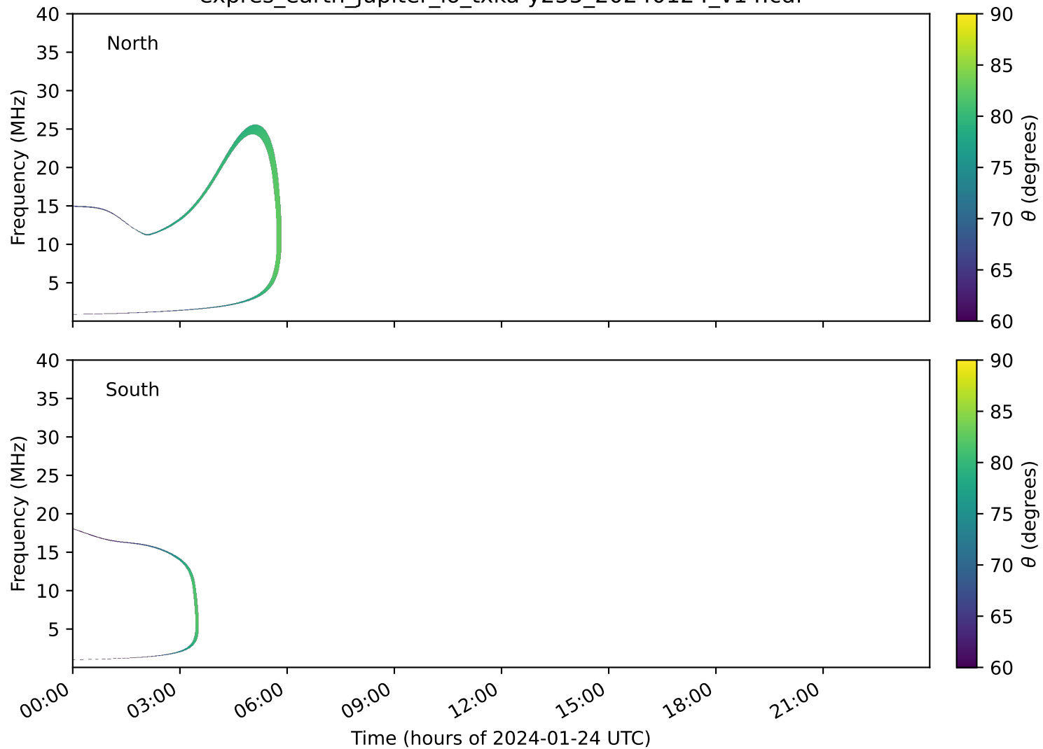
expres_earth_jupiter_io_txka-y235_20240124_v14.cdf
