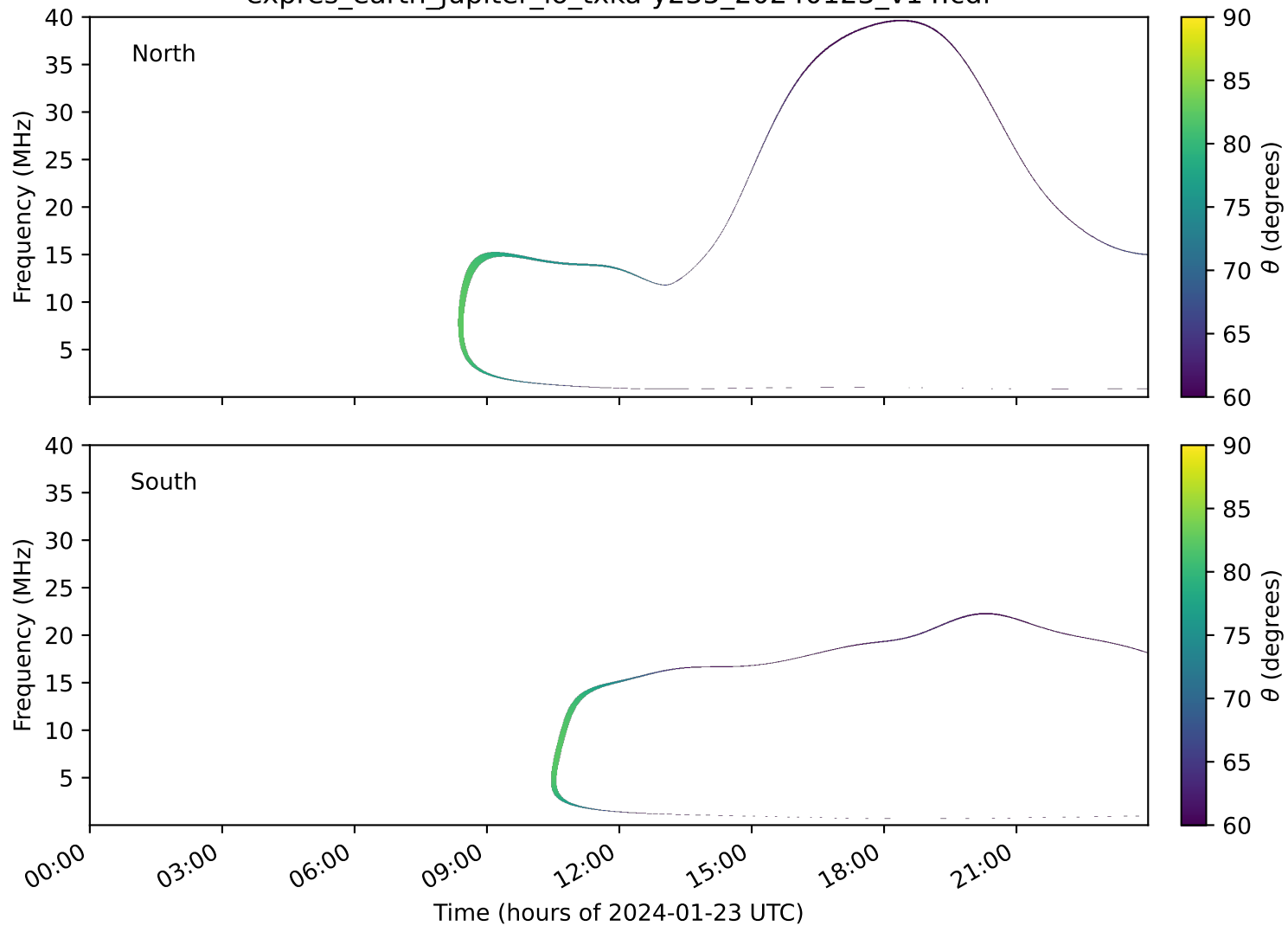
expres_earth_jupiter_io_txka-y235_20240123_v14.cdf
