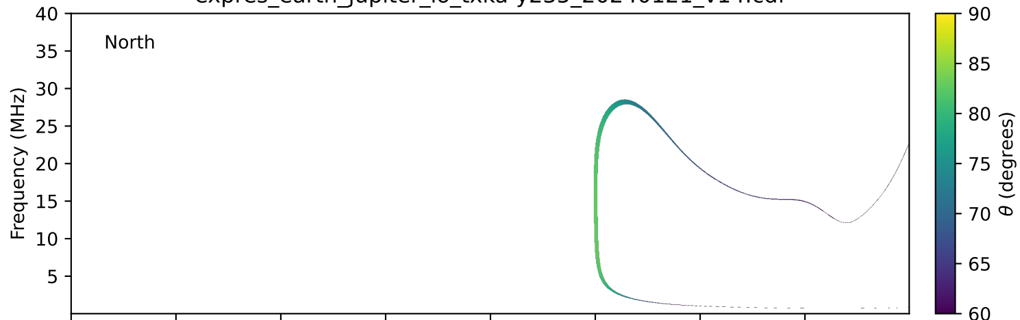
expres_earth_jupiter_io_txka-y235_20240121_v14.cdf
