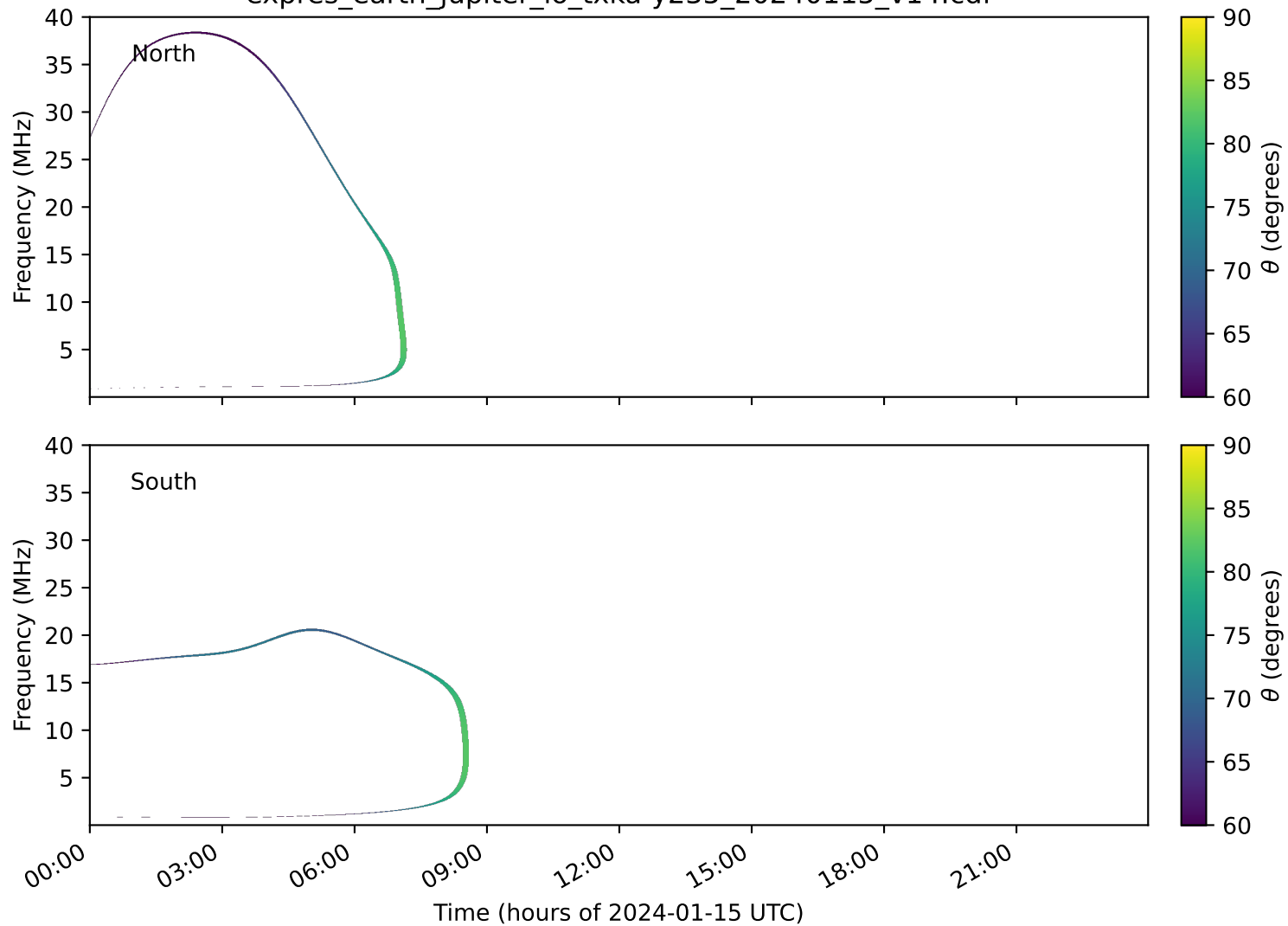
expres_earth_jupiter_io_txka-y235_20240115_v14.cdf
