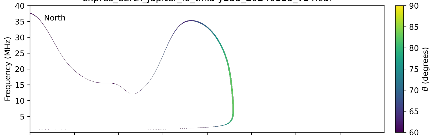
expres_earth_jupiter_io_txka-y235_20240113_v14.cdf
