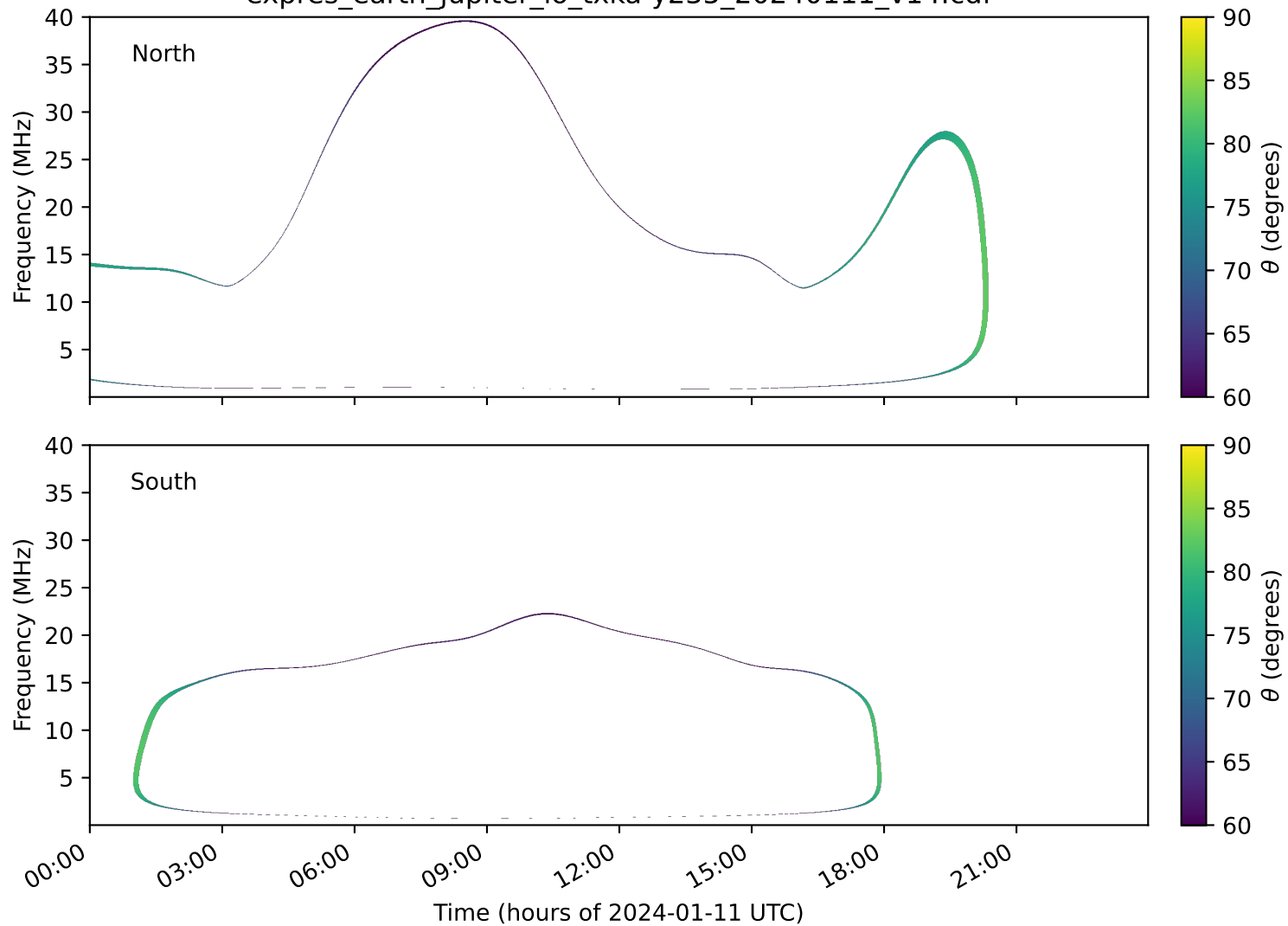
expres_earth_jupiter_io_txka-y235_20240111_v14.cdf
