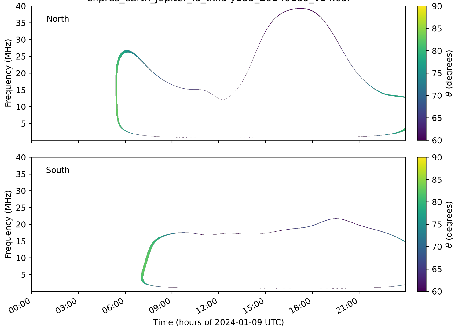
expres_earth_jupiter_io_txka-y235_20240109_v14.cdf
