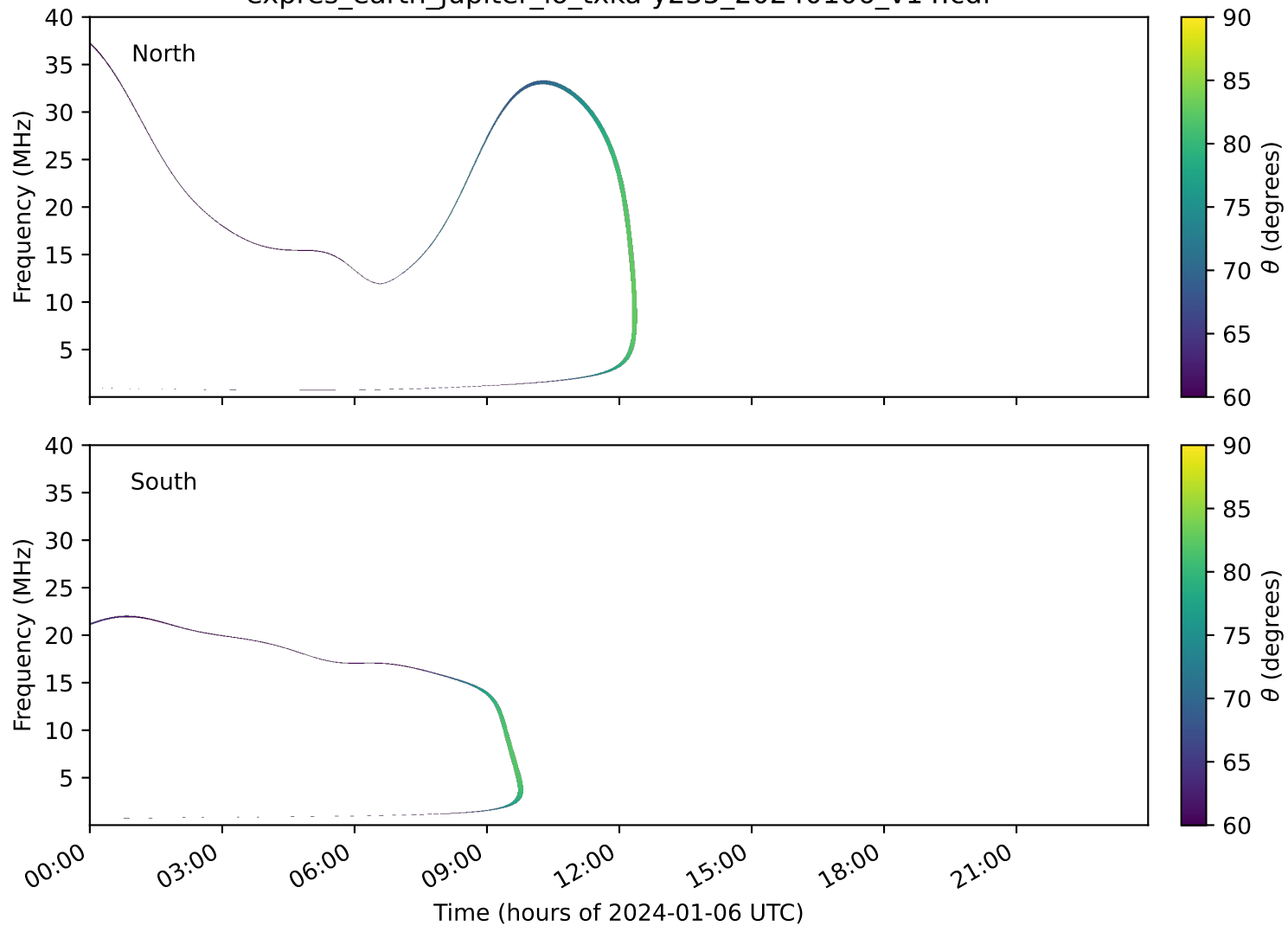
expres_earth_jupiter_io_txka-y235_20240106_v14.cdf
