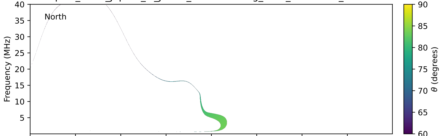
expres_earth_jupiter_io_jrm33_lossc-wid1deg_3kev_20240129_v11.cdf
