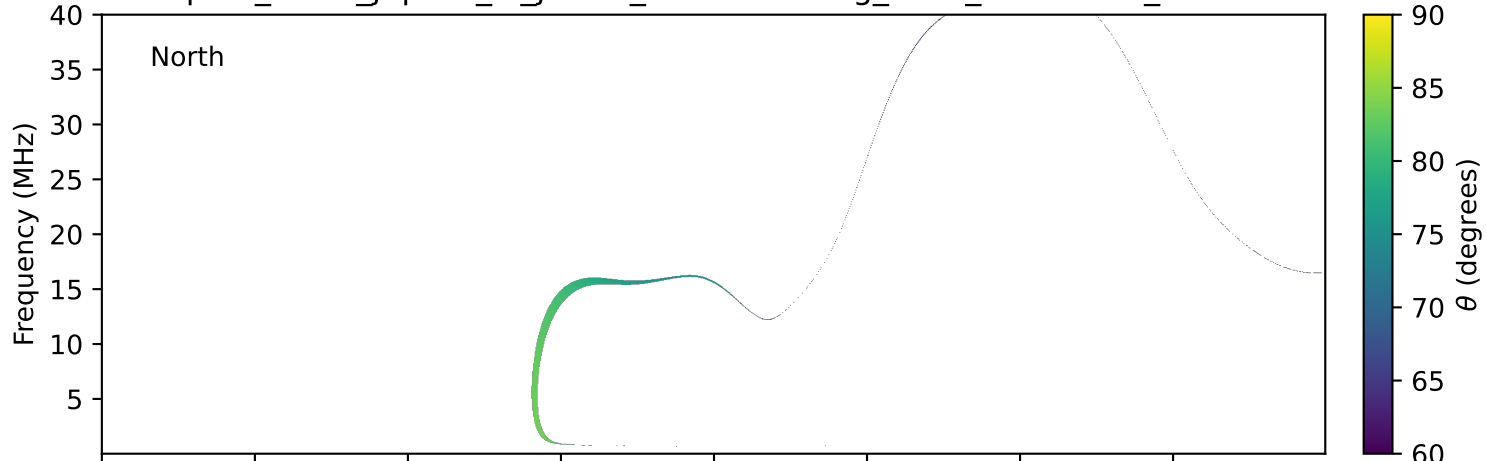
expres_earth_jupiter_io_jrm33_lossc-wid1deg_3kev_20240123_v11.cdf
