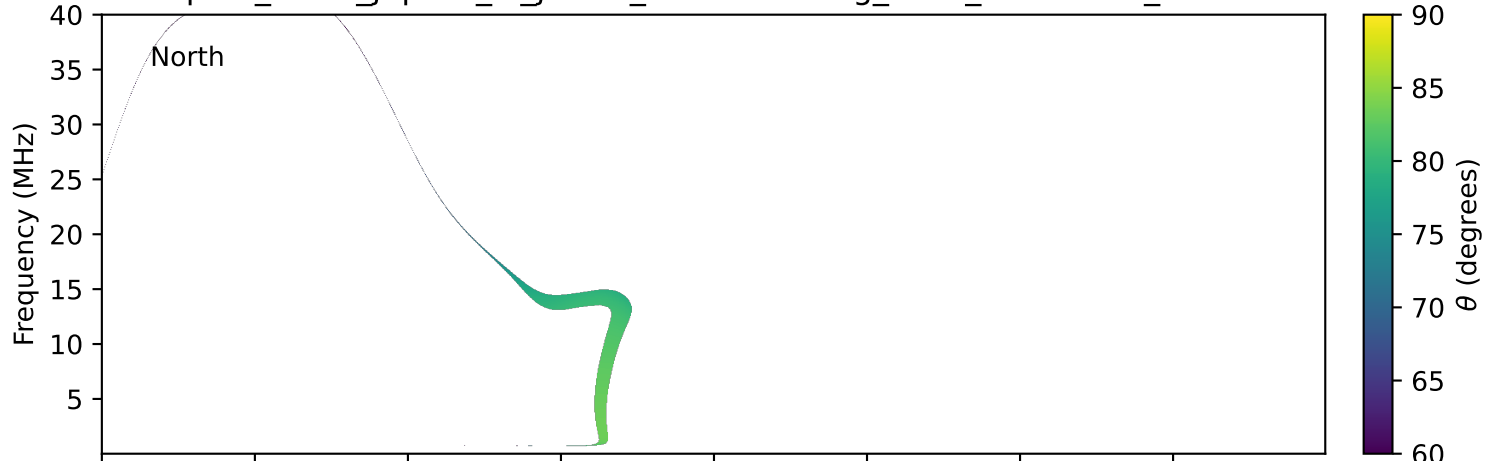
expres_earth_jupiter_io_jrm33_lossc-wid1deg_3kev_20240122_v11.cdf
