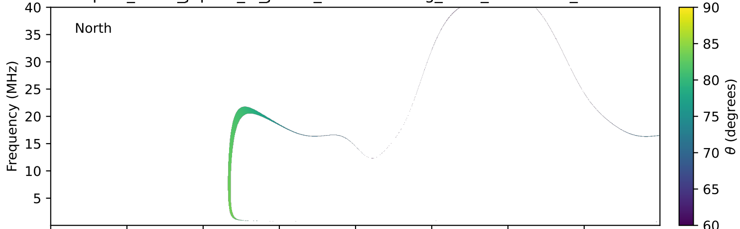
expres_earth_jupiter_io_jrm33_lossc-wid1deg_3kev_20240116_v11.cdf
