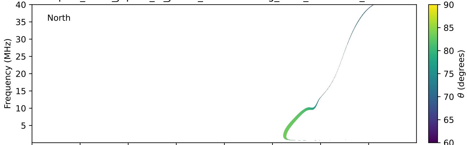
expres_earth_jupiter_io_jrm33_lossc-wid1deg_3kev_20240105_v11.cdf
