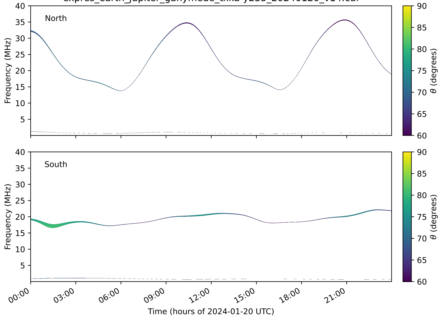
expres_earth_jupiter_ganymede_txka-y235_20240120_v14.cdf
