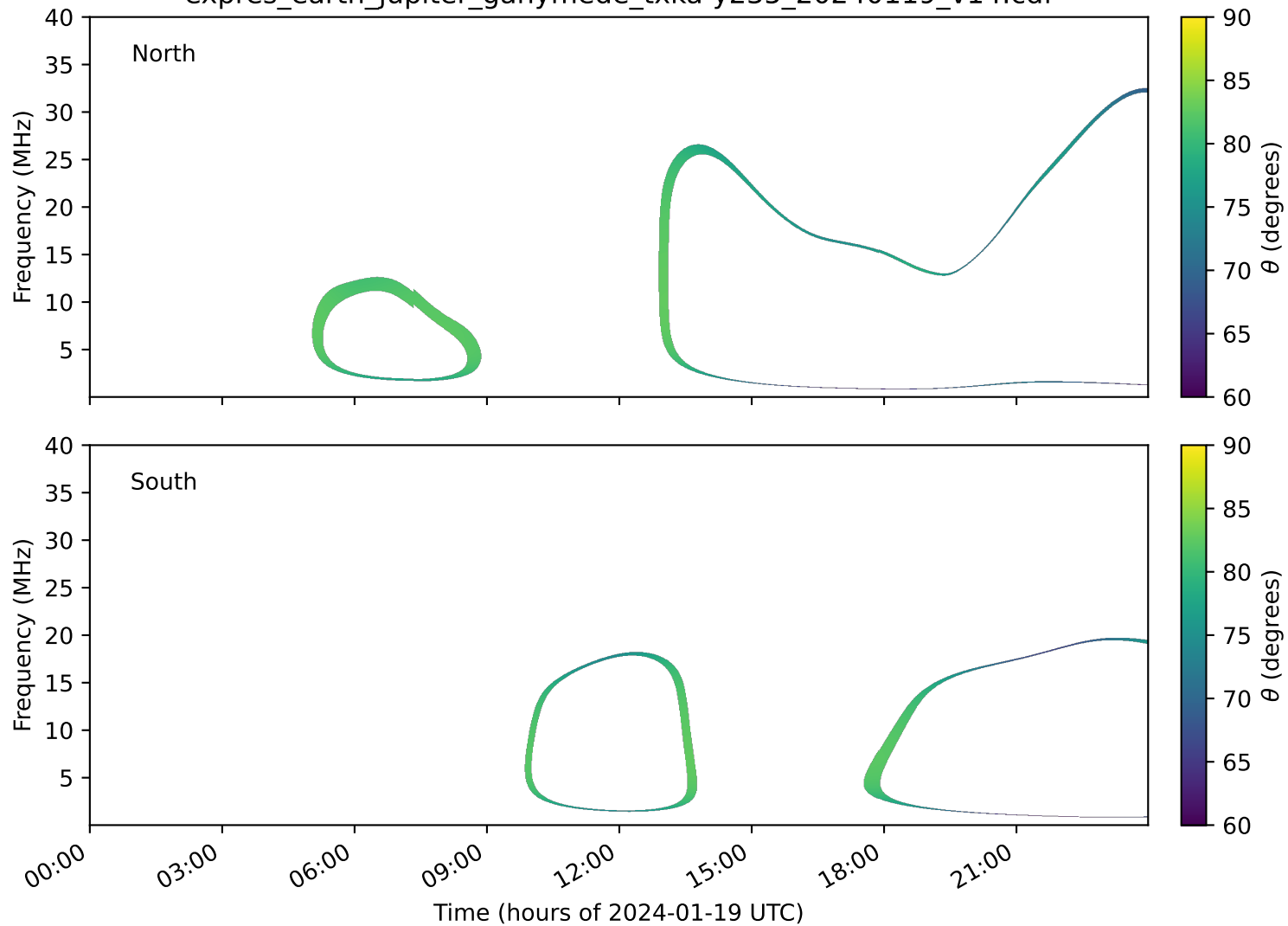
expres_earth_jupiter_ganymede_txka-y235_20240119_v14.cdf
