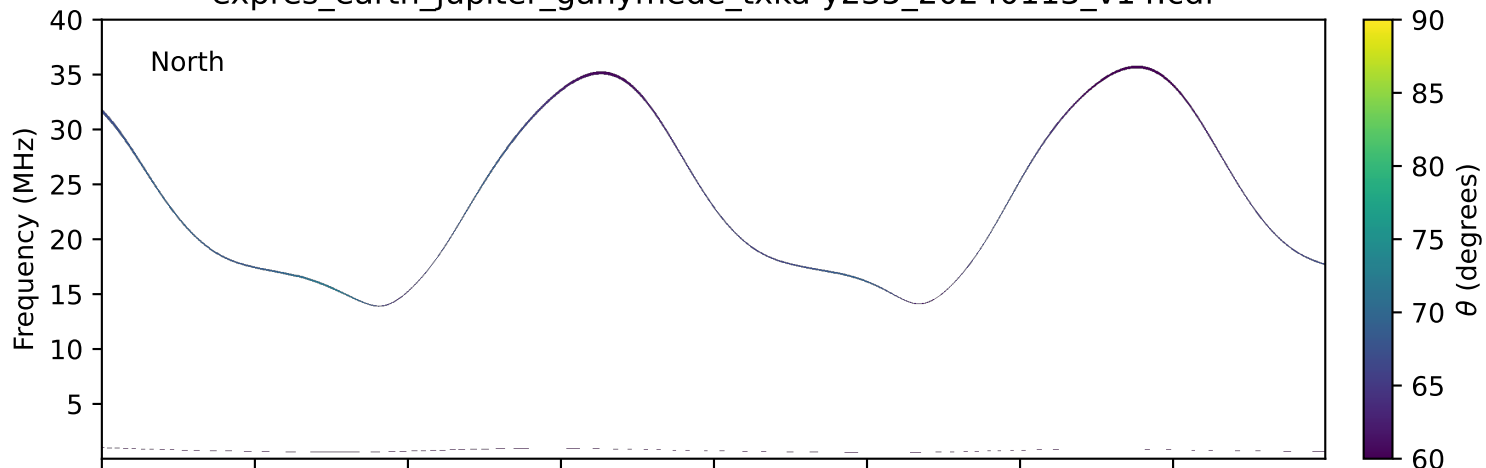
expres_earth_jupiter_ganymede_txka-y235_20240113_v14.cdf
