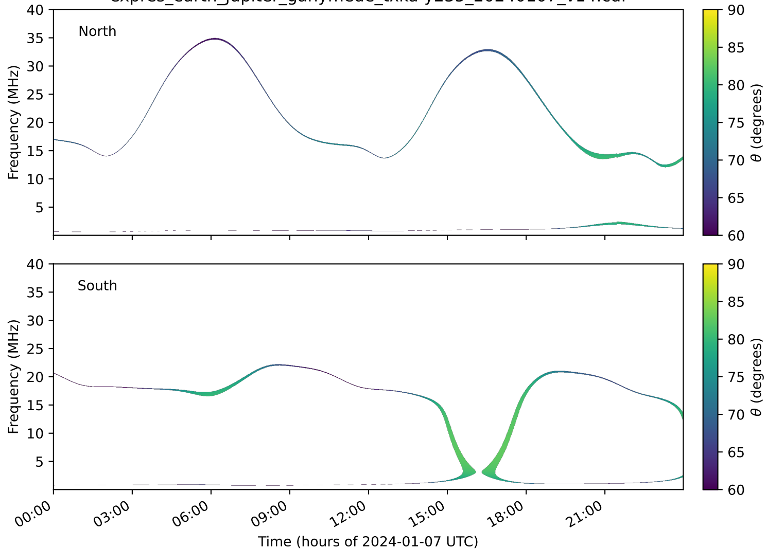
expres_earth_jupiter_ganymede_txka-y235_20240107_v14.cdf
