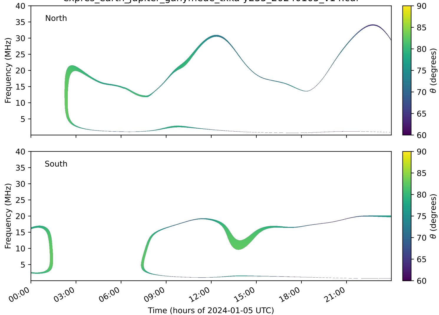
expres_earth_jupiter_ganymede_txka-y235_20240105_v14.cdf
