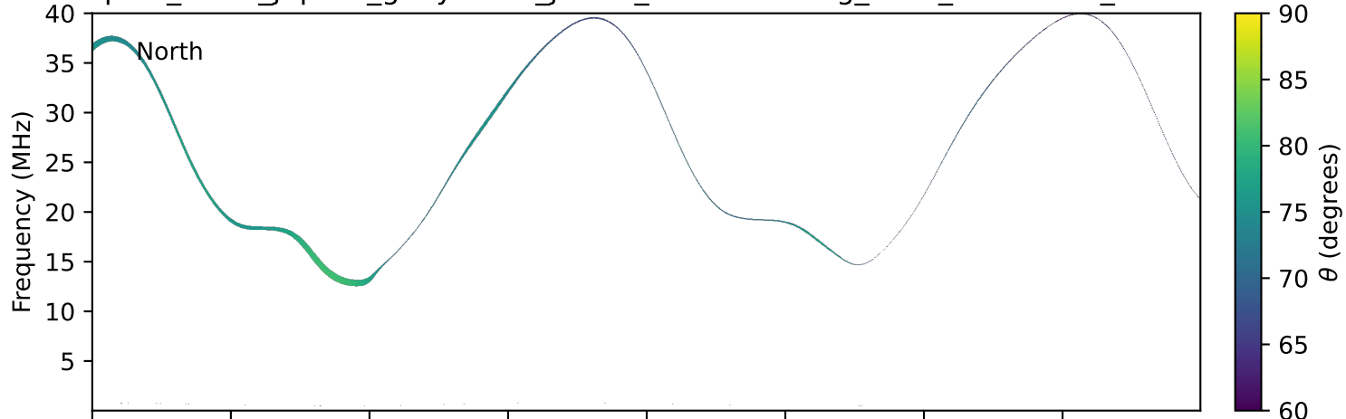
expres_earth_jupiter_ganymede_jrm33_lossc-wid1deg_3kev_20240127_v11.cdf
