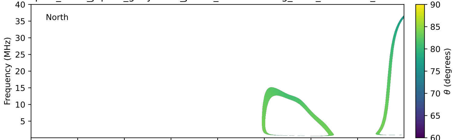
expres_earth_jupiter_ganymede_jrm33_lossc-wid1deg_3kev_20240126_v11.cdf
