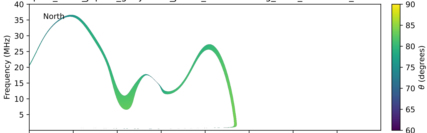
expres_earth_jupiter_ganymede_jrm33_lossc-wid1deg_3kev_20240108_v11.cdf
