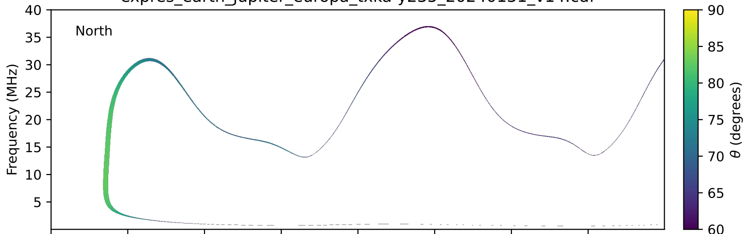
expres_earth_jupiter_europa_txka-y235_20240131_v14.cdf
