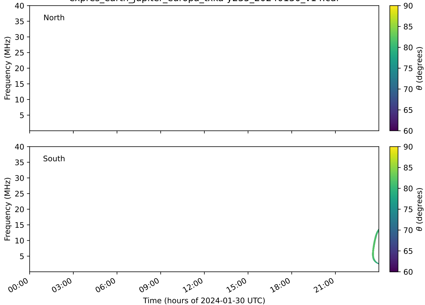
expres_earth_jupiter_europa_txka-y235_20240130_v14.cdf
