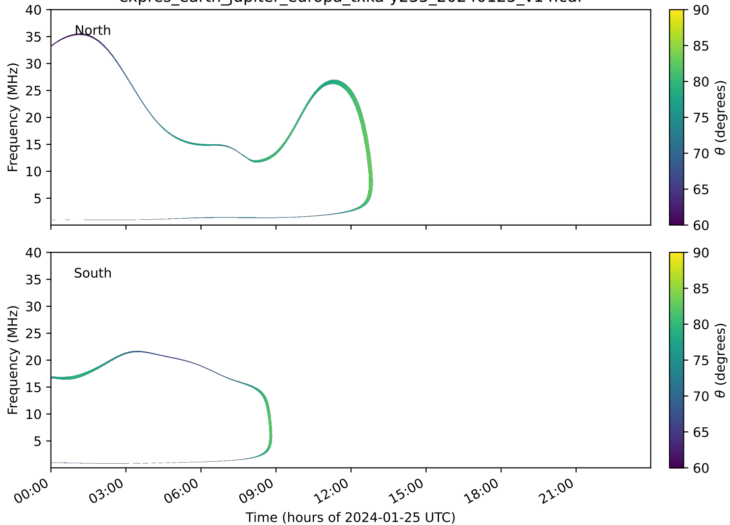
expres_earth_jupiter_europa_txka-y235_20240125_v14.cdf
