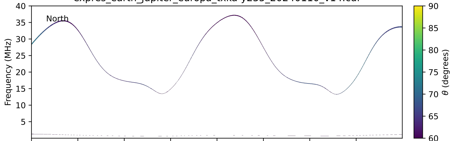
expres_earth_jupiter_europa_txka-y235_20240110_v14.cdf
