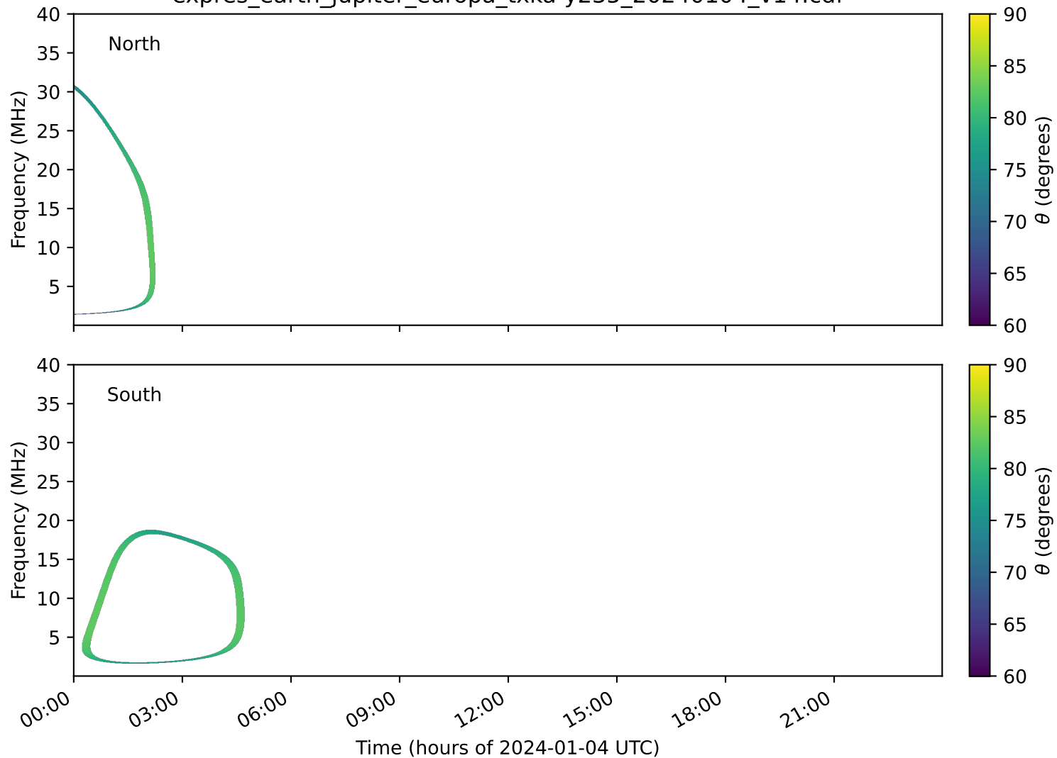
expres_earth_jupiter_europa_txka-y235_20240104_v14.cdf
