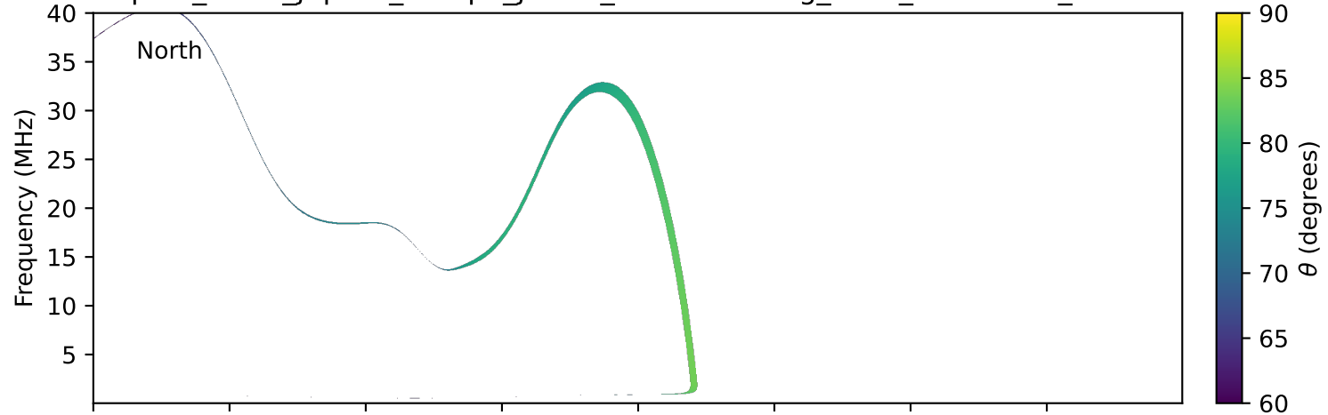
expres_earth_jupiter_europa_jrm33_lossc-wid1deg_3kev_20240125_v11.cdf
