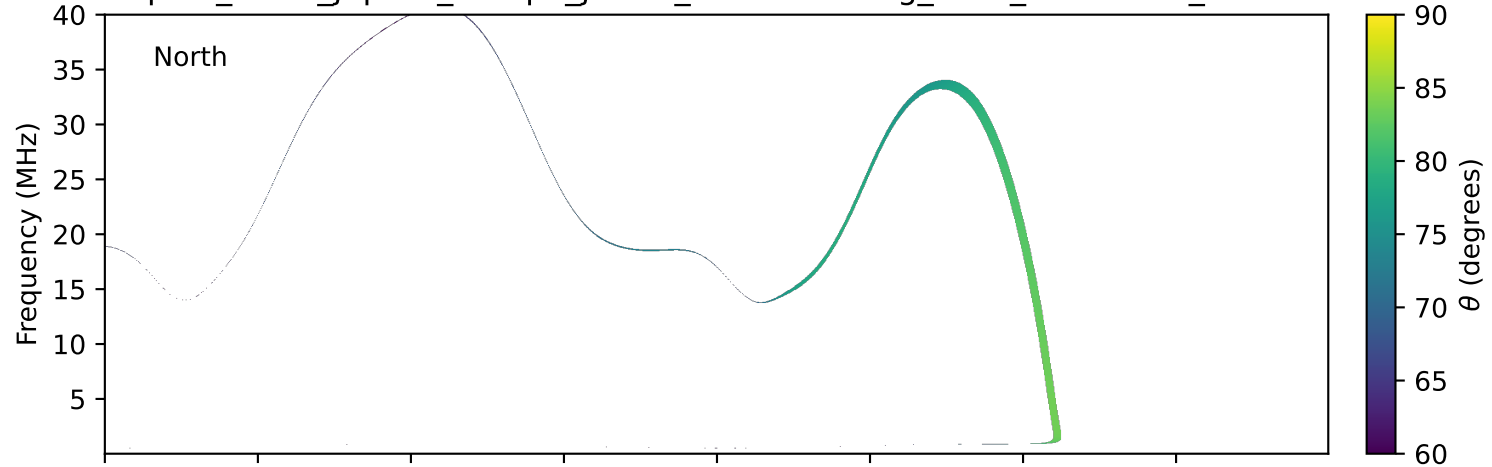
expres_earth_jupiter_europa_jrm33_lossc-wid1deg_3kev_20240107_v11.cdf
