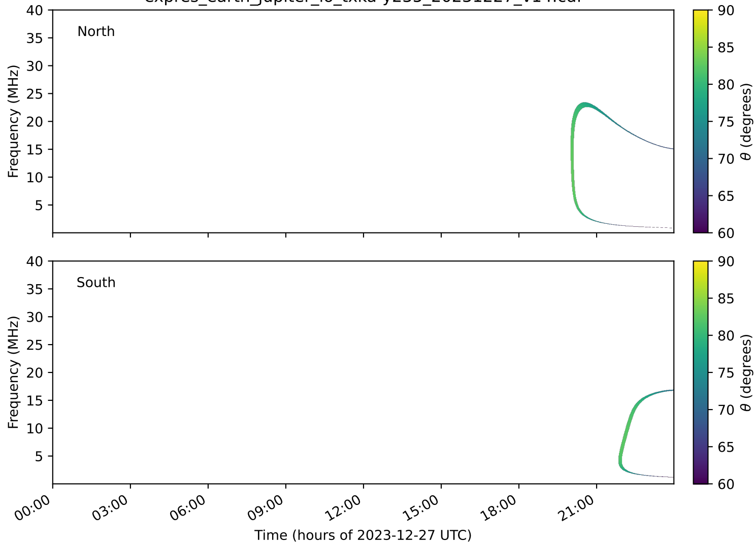
expres_earth_jupiter_io_txka-y235_20231227_v14.cdf
