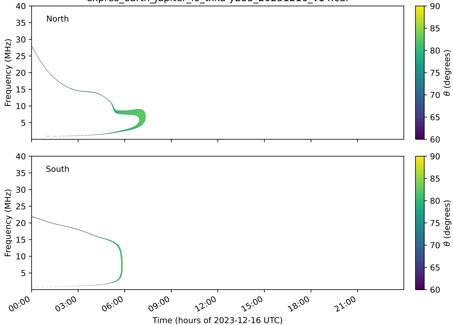
expres_earth_jupiter_io_txka-y235_20231216_v14.cdf
