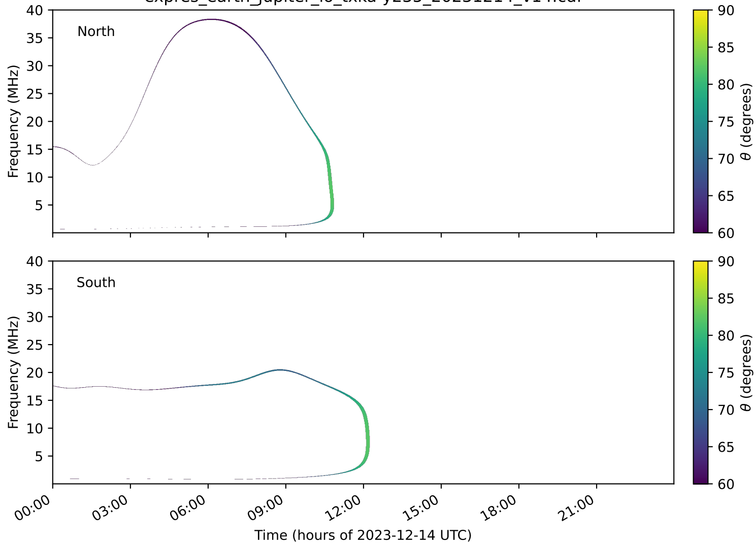
expres_earth_jupiter_io_txka-y235_20231214_v14.cdf
