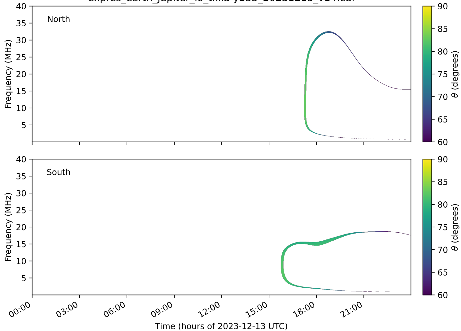
expres_earth_jupiter_io_txka-y235_20231213_v14.cdf
