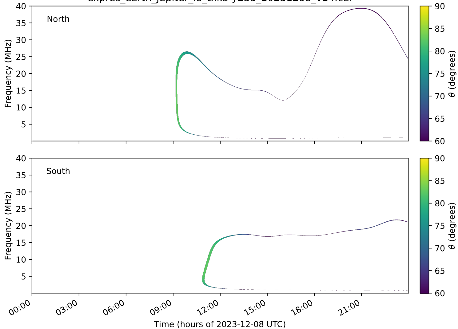
expres_earth_jupiter_io_txka-y235_20231208_v14.cdf
