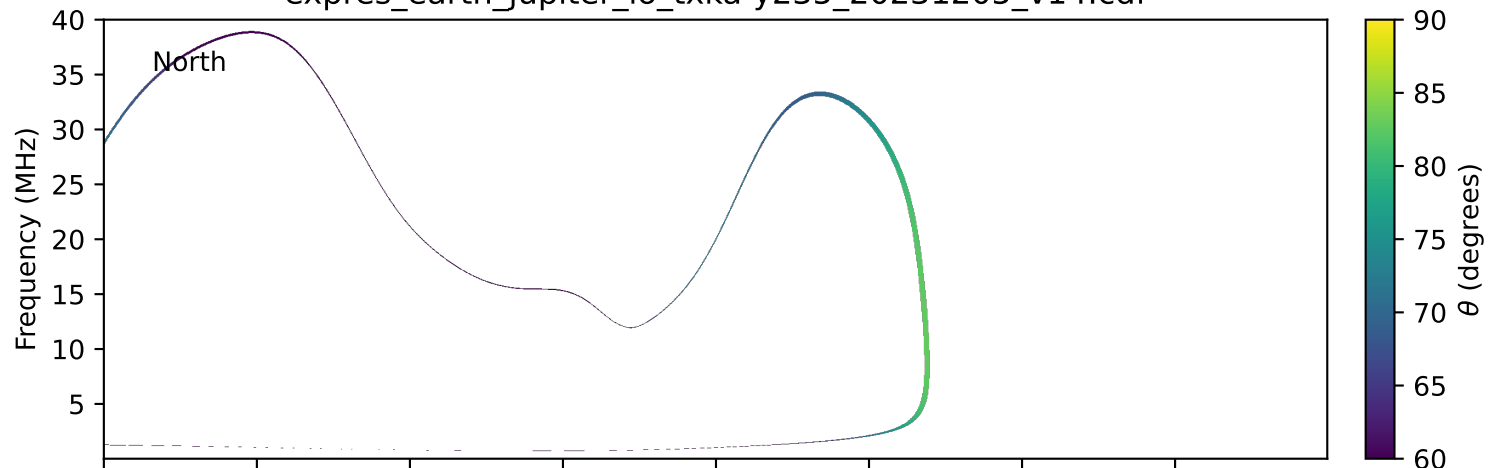
expres_earth_jupiter_io_txka-y235_20231205_v14.cdf
