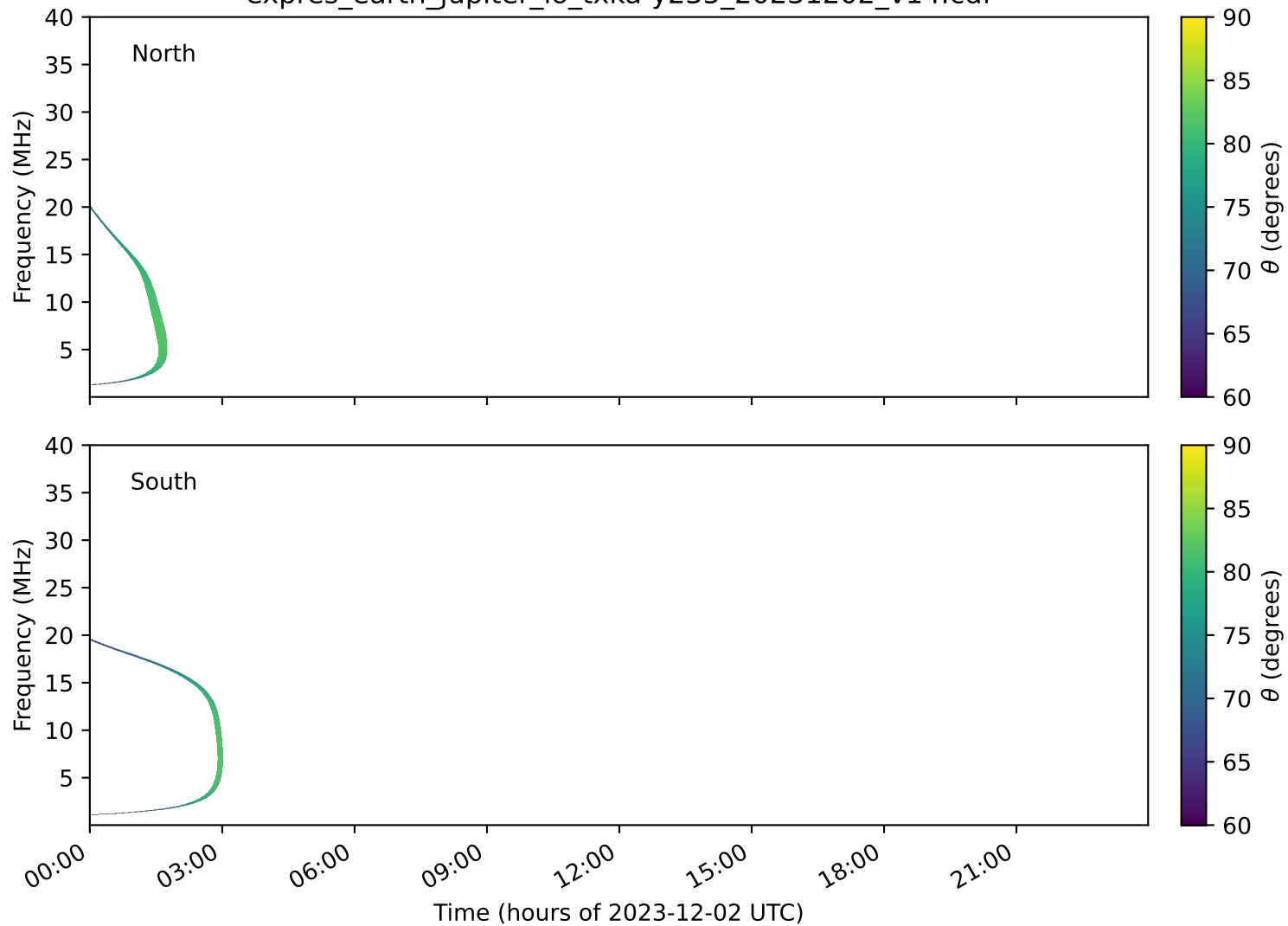
expres_earth_jupiter_io_txka-y235_20231202_v14.cdf
