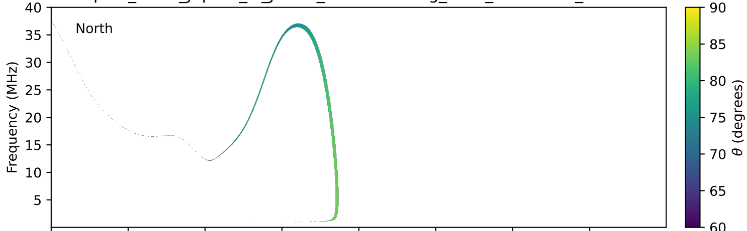
expres_earth_jupiter_io_jrm33_lossc-wid1deg_3kev_20231230_v11.cdf
