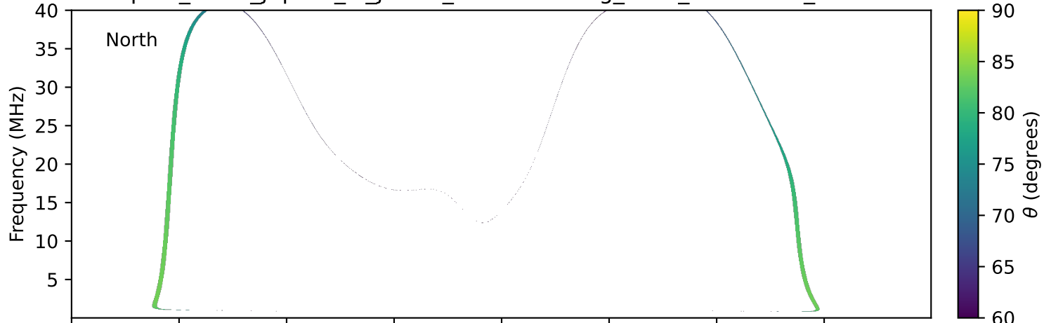
expres_earth_jupiter_io_jrm33_lossc-wid1deg_3kev_20231226_v11.cdf
