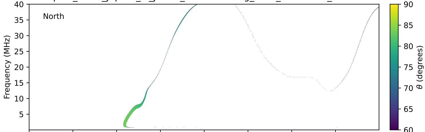
expres_earth_jupiter_io_jrm33_lossc-wid1deg_3kev_20231224_v11.cdf
