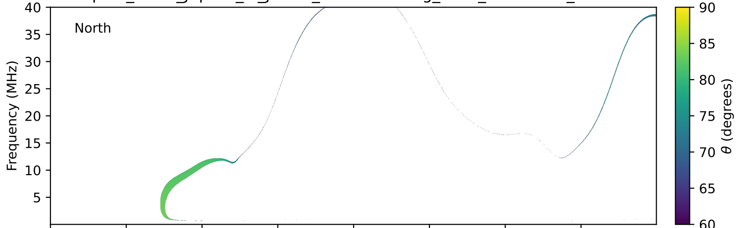
expres_earth_jupiter_io_jrm33_lossc-wid1deg_3kev_20231217_v11.cdf
