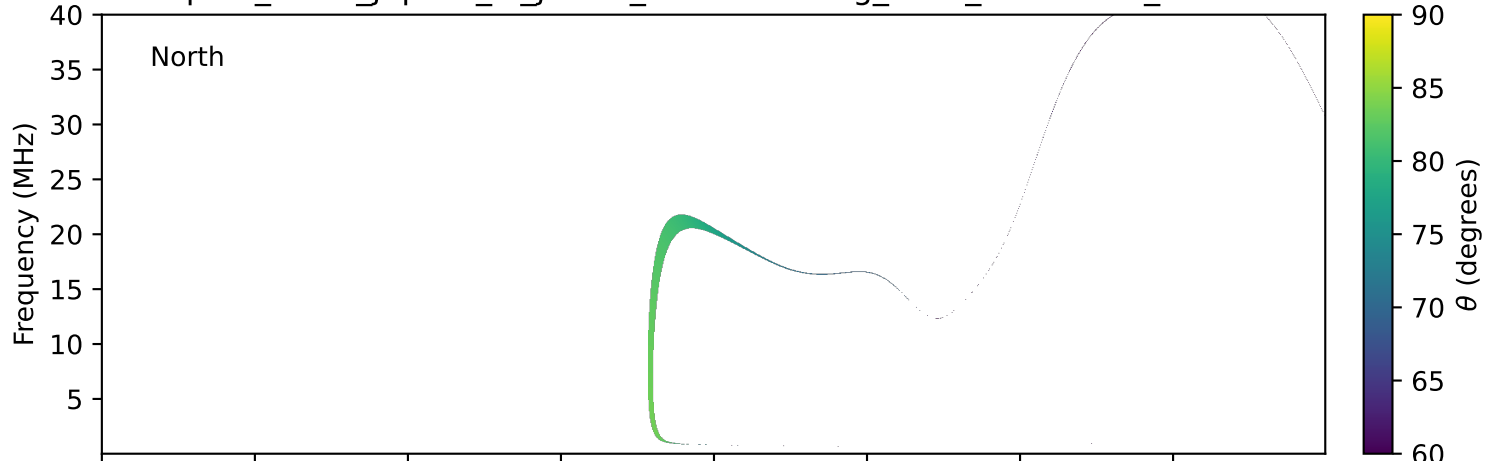
expres_earth_jupiter_io_jrm33_lossc-wid1deg_3kev_20231215_v11.cdf
