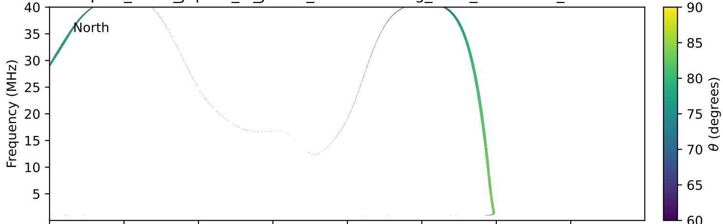
expres_earth_jupiter_io_jrm33_lossc-wid1deg_3kev_20231212_v11.cdf
