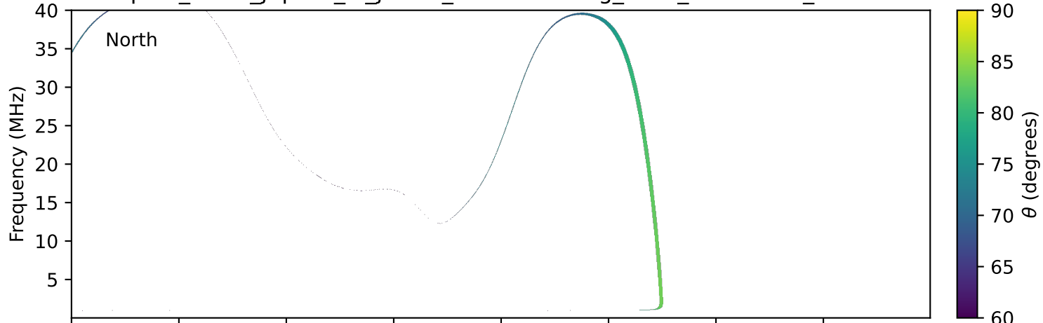
expres_earth_jupiter_io_jrm33_lossc-wid1deg_3kev_20231205_v11.cdf
