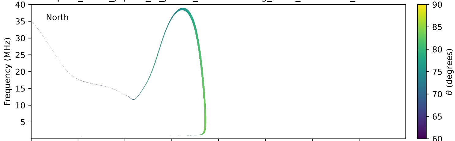
expres_earth_jupiter_io_jrm09_lossc-wid1deg_3kev_20231230_v11.cdf
