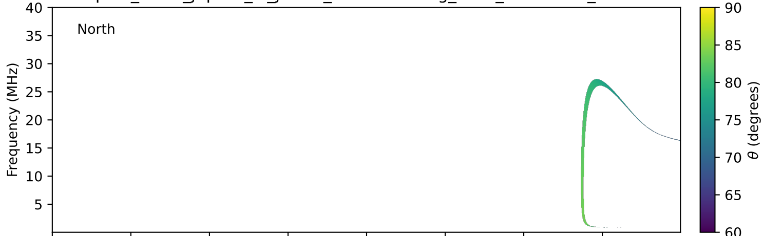
expres_earth_jupiter_io_jrm09_lossc-wid1deg_3kev_20231227_v11.cdf
