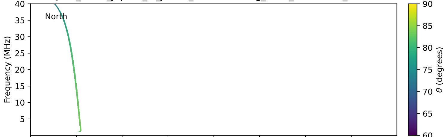
expres_earth_jupiter_io_jrm09_lossc-wid1deg_3kev_20231225_v11.cdf
