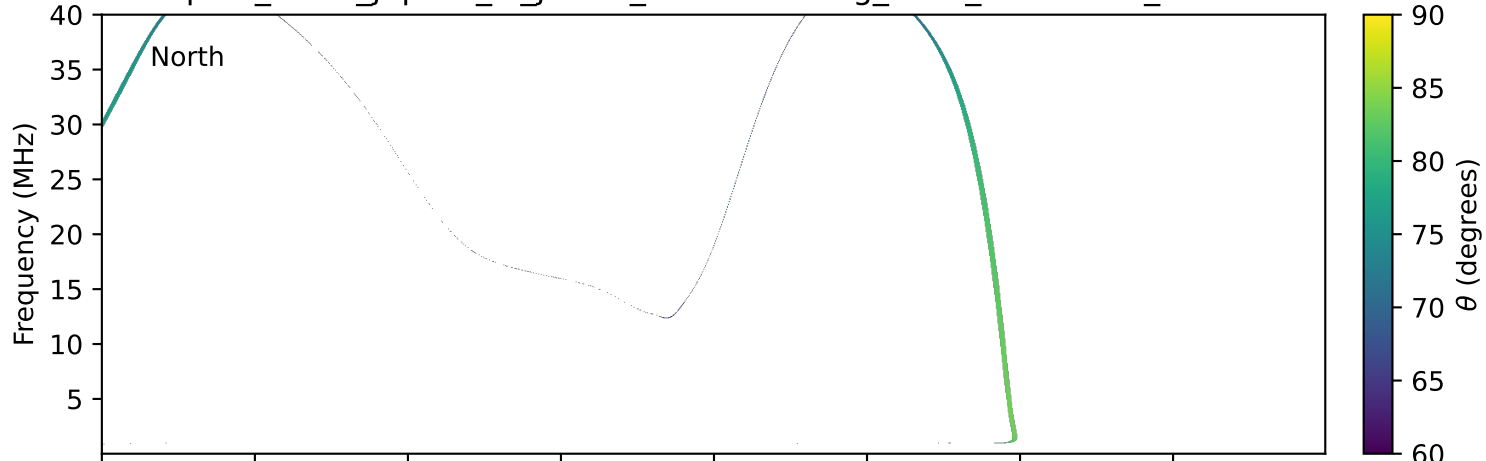
expres_earth_jupiter_io_jrm09_lossc-wid1deg_3kev_20231212_v11.cdf
