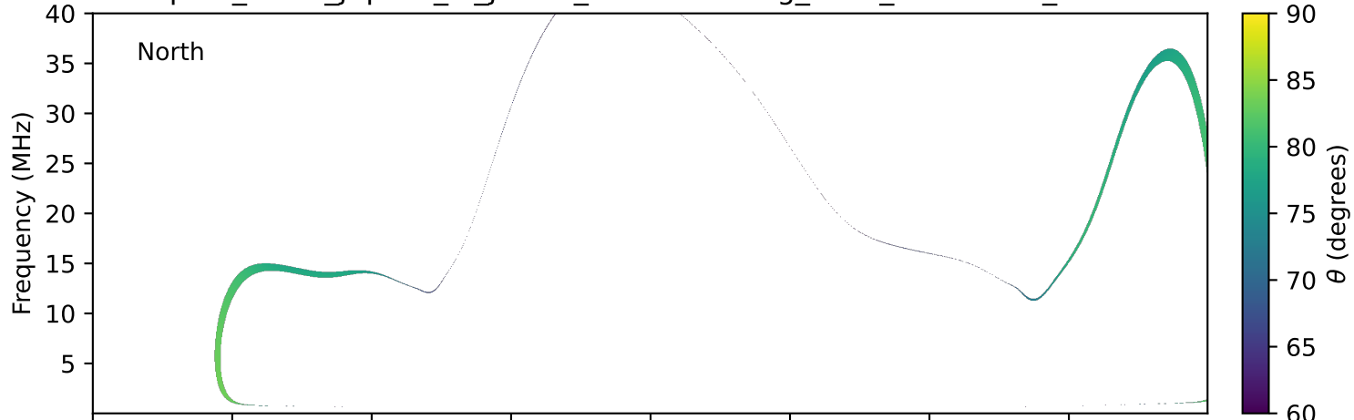
expres_earth_jupiter_io_jrm09_lossc-wid1deg_3kev_20231210_v11.cdf
