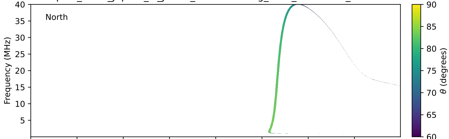
expres_earth_jupiter_io_jrm09_lossc-wid1deg_3kev_20231206_v11.cdf
