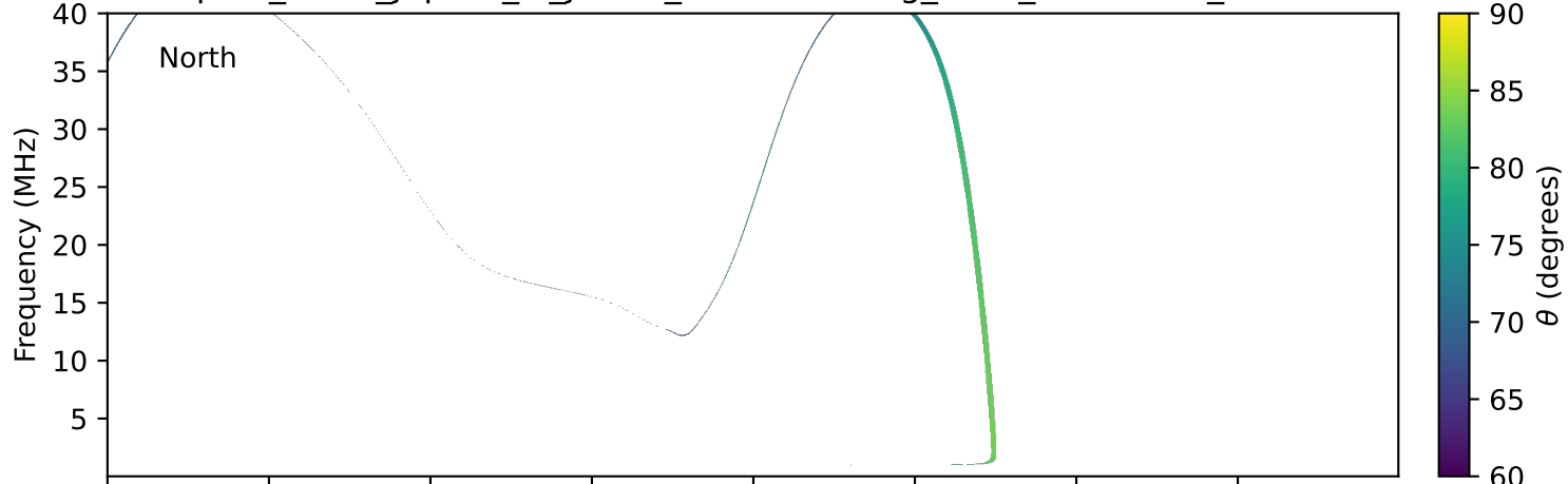
expres_earth_jupiter_io_jrm09_lossc-wid1deg_3kev_20231205_v11.cdf
